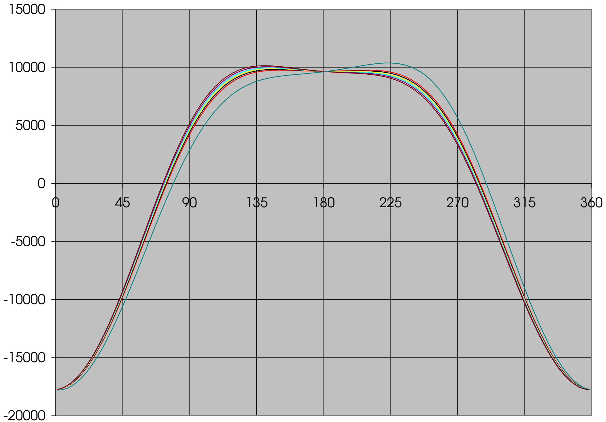
piston acceleration (m/sec 2 ) at 5000 rpm for: 0, 2, 4, 6, 8, 10 and -15 wrist-pin (or crankshaft) offset (conn-rod length:170mm, 2*crank-arm:100mm)
