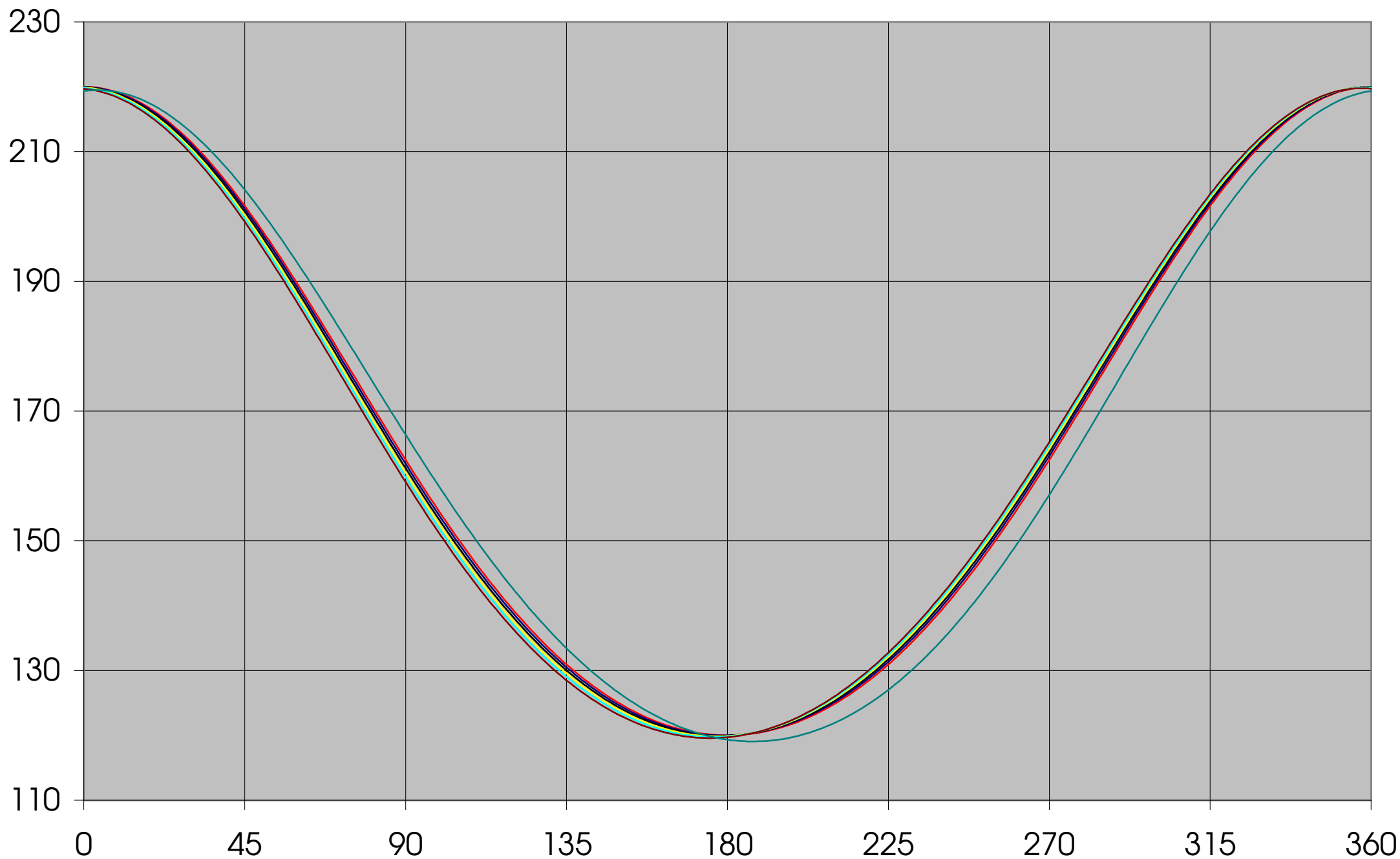
piston position (mm) for: 0, 2, 4, 6, 8, 10 and -15 wrist-pin (or crankshaft) offset (conn-rod length:170mm, 2*crank-arm:100mm)
